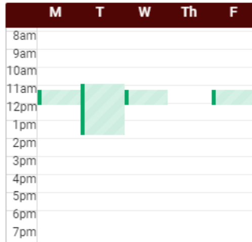
Q Open #3
