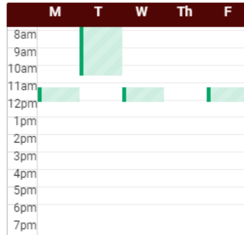
Q Open #4
