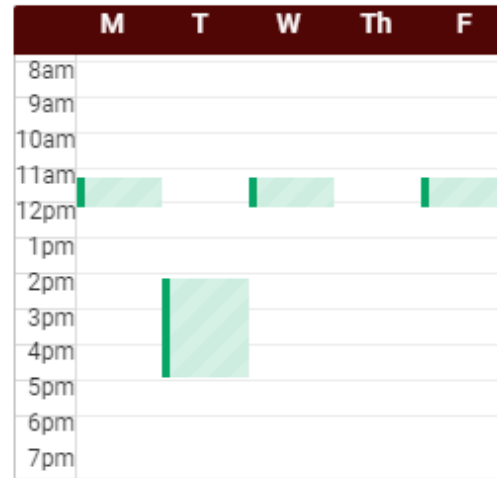
Q Open #2
