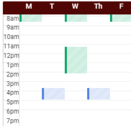
Q Open #1
